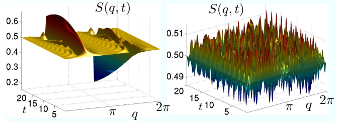
FIG. 17: Quasi-momentum distribution S(q, t) for U = 0 , L = 100 , and open (left), periodic (right) boundary conditions. Note the dramatic difference between open/periodic boundary conditions and the absence of the time-scales clearly visible for local observables as in Figs. 9, 10: The fast oscillatory behavior and the relaxation time. See Fig. 18 for S(q, t) in the presence of a trap. The non-local quantity of the quasi-momentum distribution detects the boundary conditions early.
