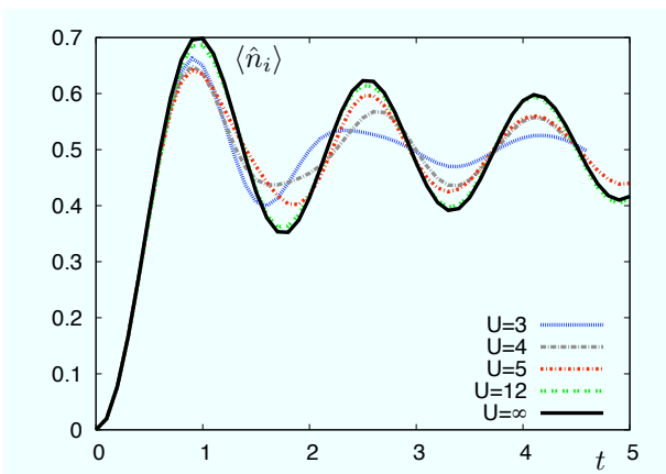
FIG. 6: Time evolution of local densities on even sites for various U compared to the limiting behavior U = \infty .
