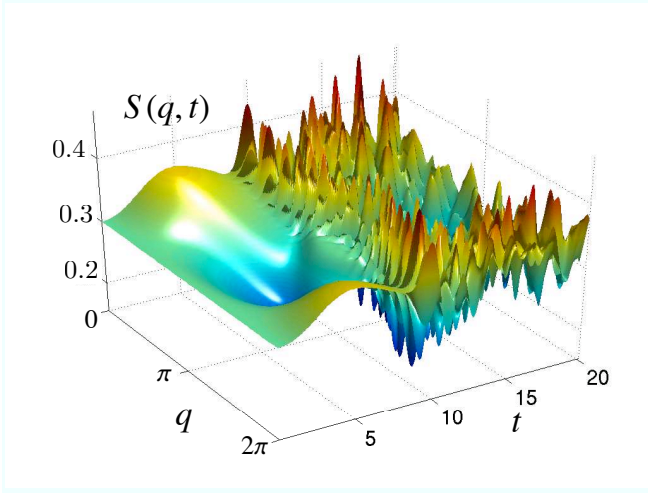
FIG. 18: Quasi-momentum distribution S(q, t) for the same parameters as in Fig. 10. Note the absence of the time-scales clearly visible for local observables as in Figs. 9, 10: The fast oscillatory behavior and the relaxation. The recurrence is however clearly visible.
