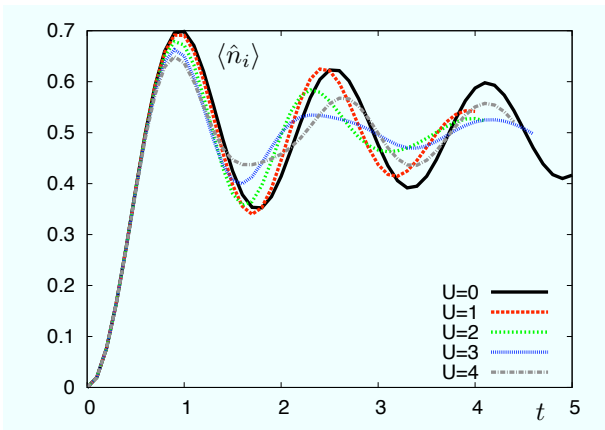
FIG. 5: Time evolution of local densities on even sites for various U compared to the limiting behavior U = 0 .
