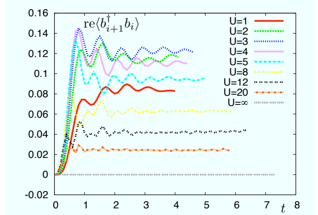
FIG. 11: Real part of correlations to neighbors \langle \hat{b}_{i+1}^\dagger(t) \hat{b}_i(t) \rangle as a function of time, for different values of U . Note that in the effectively free cases U = 0 and U = \infty , the absolute value of these correlators converges to zero.
