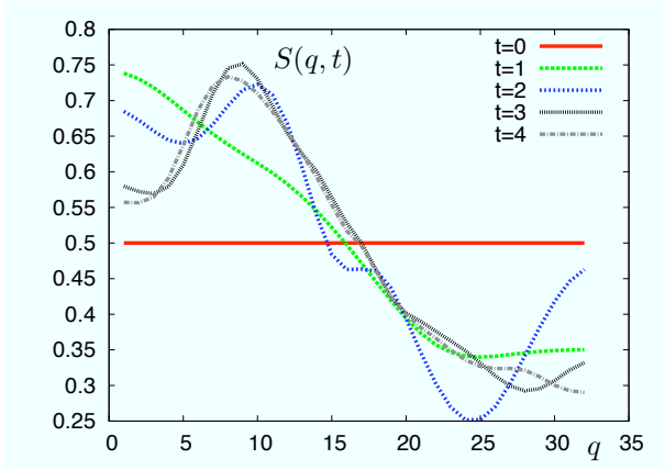
FIG. 15: Quasi-momentum distribution as a function of time, for U = 1.5 . The labels q on the x -axis correspond to momenta \pi/(L+1)q , best suited to DMRG open boundary conditions, as explained in the text.
