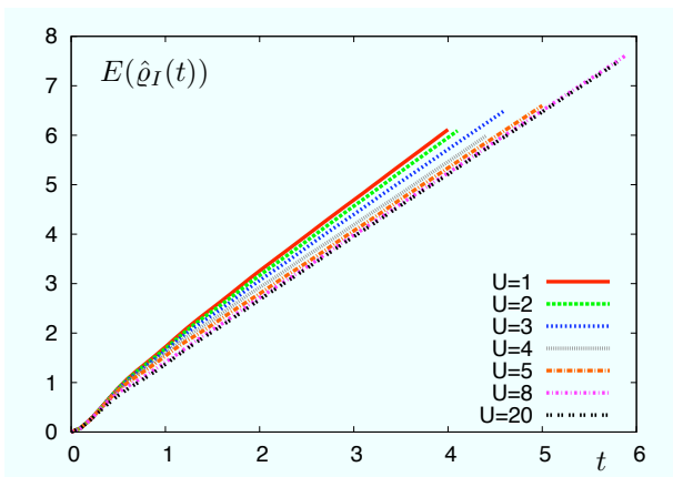
FIG. 20: Von-Neumann entropy of the bisected half-chain between sites \{1, \dots, 16\} and \{17, \dots, 32\} vs. time for various interaction strengths U .
