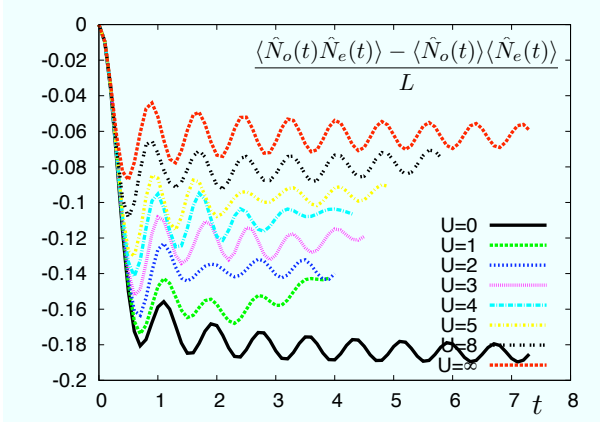
FIG. 19: Global density-density correlations for a system of length L = 32 for various interaction strengths U .
