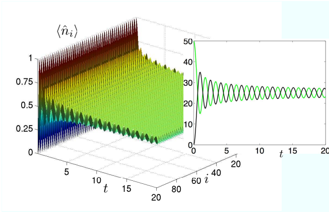
FIG. 9: Density \langle \hat{n}_i(t) \rangle (left) for U = 0 , L = 100 , and periodic boundary conditions. The plot on the right shows \langle \hat{N}_e(t) \rangle (black) and \langle \hat{N}_o(t) \rangle (green), compare Fig. 10, where the same is shown including a trapping potential.
