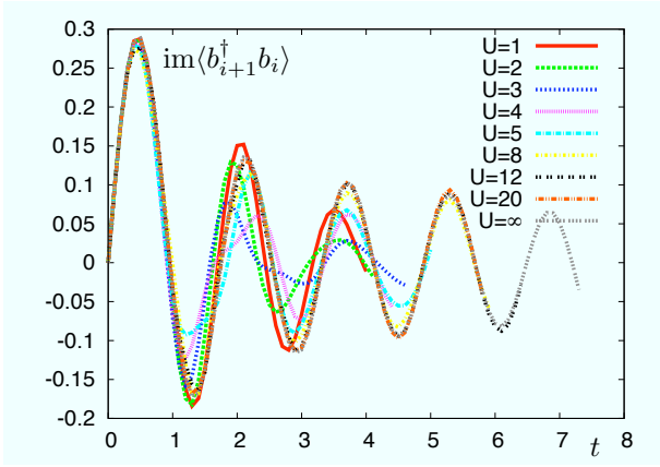
FIG. 12: Imaginary part of correlations to neighbors \langle \hat{b}_{i+1}^\dagger(t) \hat{b}_i(t) \rangle as a function of time, for different values of U .
