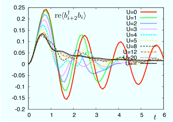
FIG. 14: Real part of correlations to neighbors \langle \hat{b}_{i+2}^\dagger(t)\hat{b}_i(t) \rangle as a function of time, for different values of U .
