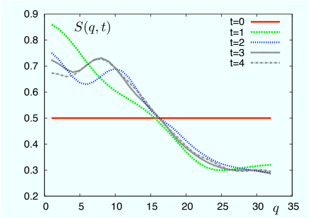
FIG. 16: Quasi-momentum distribution as a function of time, for U = 3 , marking the cross-over regime. Labels as in Fig. 15.
