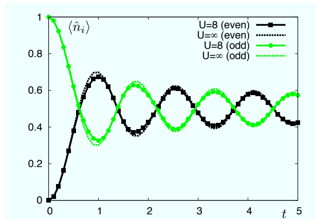
FIG. 4: Local density \langle \hat{n}_i(t) \rangle vs. time, showing local relaxation. Shown is the time evolution of an even and an odd site for U = 8 and U = \infty . The agreement is almost perfect.
