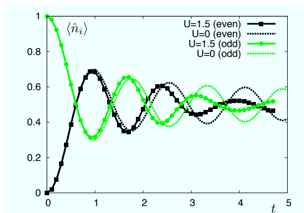
FIG. 2: Local density \langle \hat{n}_i(t) \rangle vs. time, showing local relaxation. Shown is the time evolution of an even and an odd site for U = 0 and U = 1.5 .
