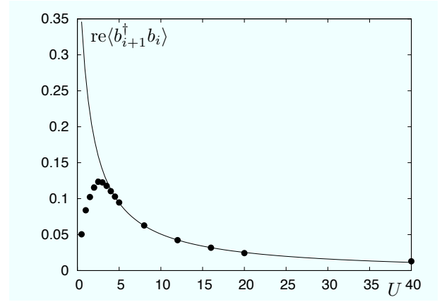
FIG. 13: Equilibrated value of the real part of correlations to neighbors \langle \hat{b}_{i+1}^\dagger(t) \hat{b}_i(t) \rangle for large t for different values of U . As a guide to the eye, large- U behavior is fitted by a solid line proportional to 1/U .
