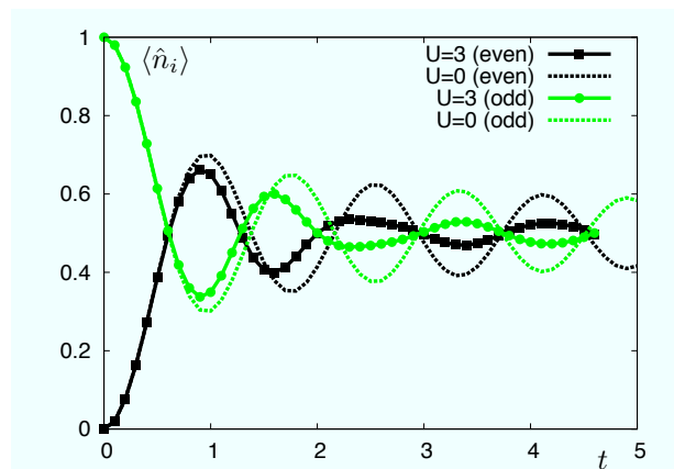
FIG. 3: Local density \langle \hat{n}_i(t) \rangle vs. time, showing local relaxation. Shown is the time evolution of an even and an odd site for U = 0 and U = 3 . Note the strong deviation from the non-interacting limit and the strong suppression of density oscillations.
