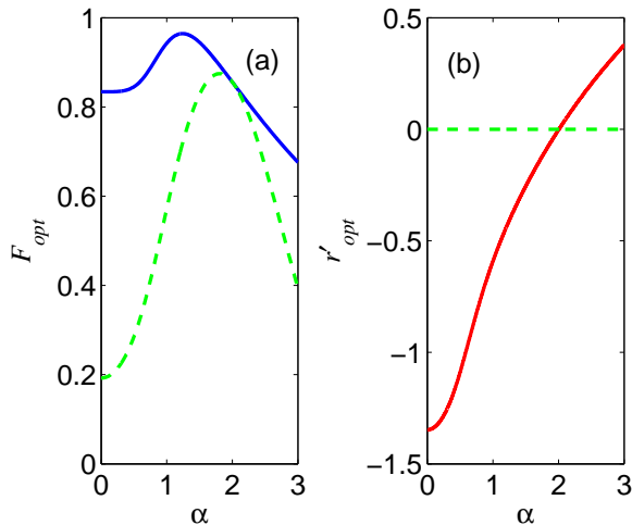
FIG. 5: (a) Optimal fidelity F_{opt} between the TPSS ( a^2 ) generated using ideal avalanche photon detectors and the SSCS of amplitude \alpha (solid curve) and the optimal fidelity with the corresponding regular SCS (dashed curve). The squeezing parameter of the initial squeezed state is r = -0.7 . The parameter of real transformation is T = 0.99 . (b) The squeezing parameter of the target SSCS for which the fidelity is optimized.
