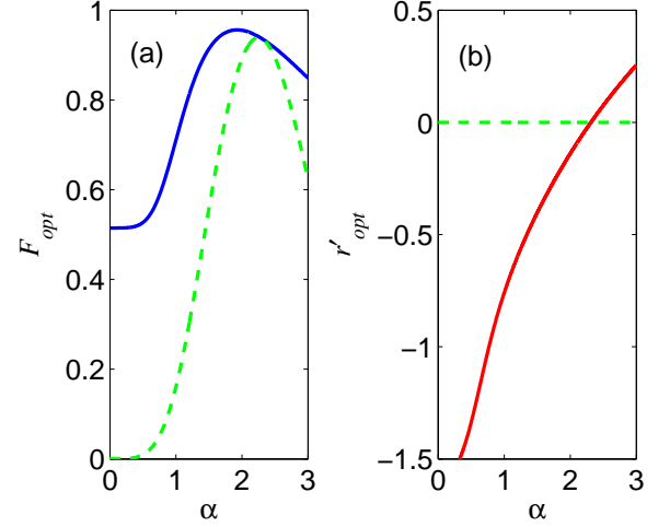
FIG. 2: (a) Optimal fidelity F_{opt} between the ideal PSAS ( a^\dagger a ) and the SCS of amplitude \alpha (solid curve) and the optimal fidelity between the ideal PSAS and the corresponding regular SCS (dashed curve). The squeezing parameter r'_{opt} of the initial squeezed state is r = -0.7 . (b) The squeezing parameter of the target SCS for which the fidelity is optimized.
