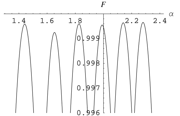
FIG. 9: The optimal fidelity between the NPSSs with \mathcal{R}(= T \tanh r) = 0.6 and the SSCSs of r' = 0.44 from N = 3 (left) to N = 8 (right). The x axis represents the amplitude \alpha of the target SSCS. The optimal fidelity is F > 0.999 regardless of the number of N .
