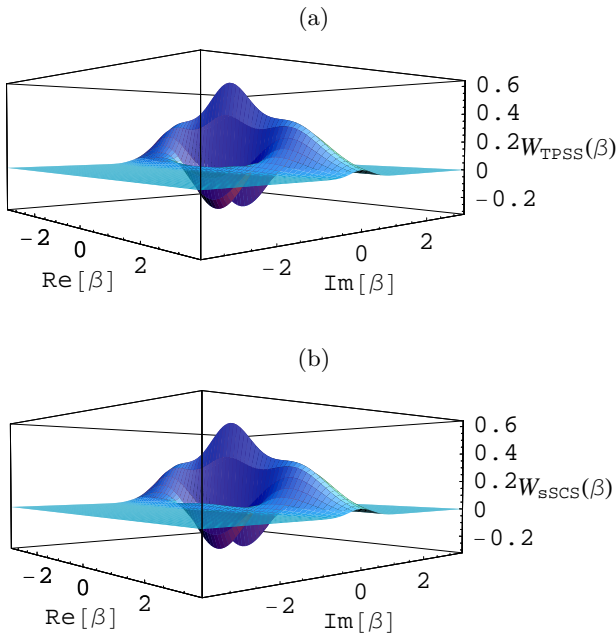
FIG. 3: (a) The Wigner function of the TPSS with r = -0.7 ( \approx 6.1\text{dB} ) and (b) the Wigner function of the ideal SSCS with \alpha = 1.26 and r' = -0.425 . The fidelity between the two states is nearly perfect as F > 0.999 .
