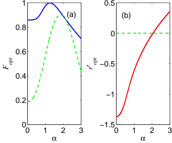
FIG. 1: (a) Optimal fidelity F_{opt} between the ideal TPSS ( a^2 ) and the squeezed SCS of amplitude \alpha (solid curve) and the optimal fidelity between the ideal TPSS and the corresponding regular SCS (dashed curve). The squeezing parameter r'_{opt} of the initial squeezed state is r = -0.7 . (b) The squeezing parameter r' of the target SCS for which the fidelity is optimized.
