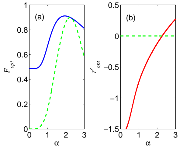
FIG. 6: Optimal fidelity F_{opt} between the PSAS ( a^\dagger a ) generated using ideal avalanche photon detectors and the SSCS of amplitude \alpha (solid curve) and the optimal fidelity with the corresponding regular SCS (dashed curve). The squeezing parameter of the initial squeezed state is r = -0.7 . (b) The squeezing parameter of the target SSCS for which the fidelity is optimized. The parameters of real transformations are T = 0.99 , G = 1.01 .
