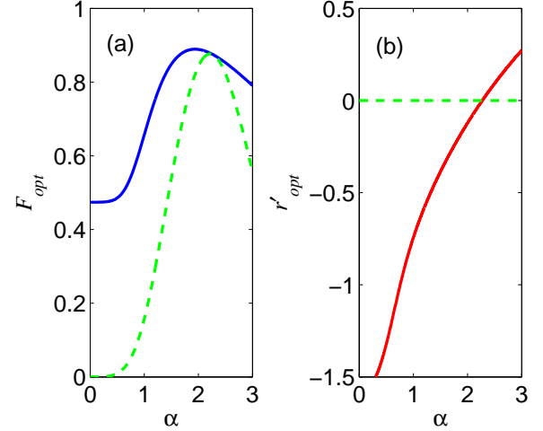
FIG. 8: (a) Optimal fidelity F_{opt} between the PSAS ( a^\dagger a ) generated using realistic avalanche photon detectors and the SSCS of amplitude \alpha (solid curve) and the optimal fidelity with the corresponding regular SCS (dashed curve). The squeezing parameter of the initial squeezed state is r = -0.7 . (b) The squeezing parameter of the target SSCS for which the fidelity is optimized. The parameters of realistic transformations are T = 0.99 , G = 1.01 and \eta = 0.6 .
