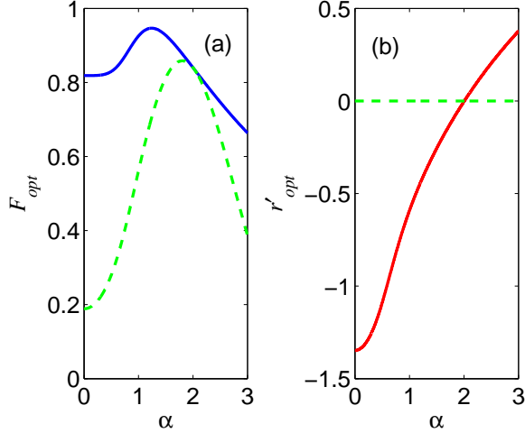
FIG. 7: (a) Optimal fidelity F_{opt} between the TPSS ( a^2 ) generated using realistic avalanche photon detectors and the SSCS of amplitude \alpha (solid curve) and the optimal fidelity with the corresponding regular SCS (dashed curve). The squeezing parameter of the initial squeezed state is r = -0.7 . The parameters of realistic transformations are T = 0.99 and \eta = 0.6 . (b) The squeezing parameter of the target SSCS for which the fidelity is optimized.
