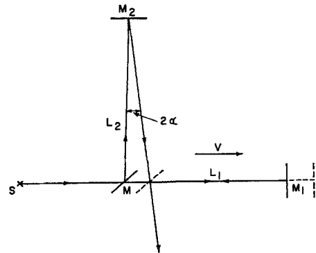
FIG. 4. Michelson experiment.
