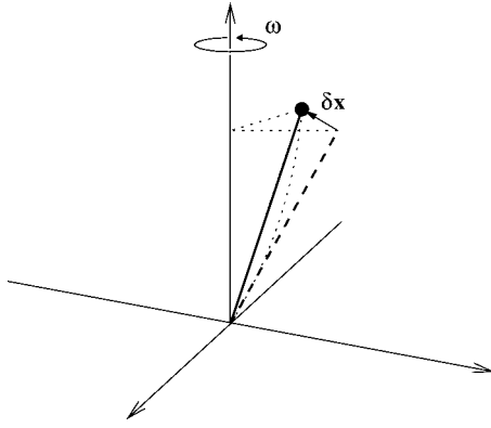
Fig. 16. A particle (the black dot) moving along a rotating straight line (depicted at two successive time steps—the dashed and the solid line), as observed relative to an inertial system S . Relative to S the particle trajectory (the dotted line) curves.
