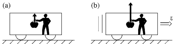
Fig. 2. A train on a platform with a constant proper acceleration a upward. (a) The train is at rest; (b) the train is moving relative to the platform. The force required of a man on the train to keep an apple at a fixed height is higher when the train moves than when it is at rest relative to the platform.
