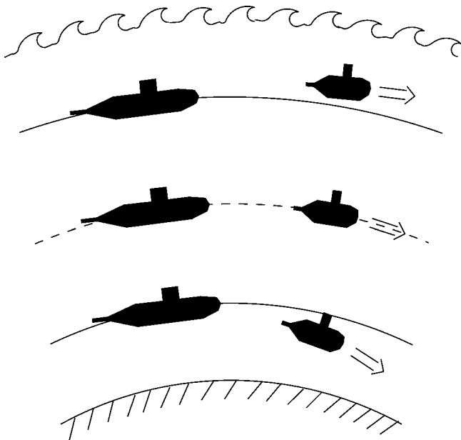
Fig. 12. Submarines moving at different depths in the ocean of an imaginary very dense planet. The dashed line is the photon radius. The submarines outside the photon radius will float upward if they are given an azimuthal velocity; the opposite holds within the photon radius.
