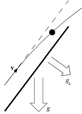
Fig. 6. A particle moving along a trajectory of curvature R relative to the accelerating reference frame. The thick line is freely falling and is initially ( t=0 ) aligned with the dashed line. For forces perpendicular to the direction of motion, only the perpendicular part of the acceleration \mathbf{g} is relevant.
