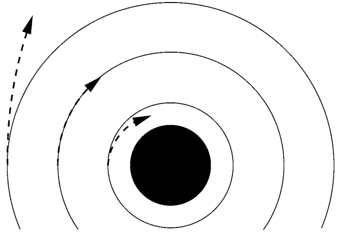
Fig. 7. Trajectories of geodesic photons (dashed curves) relative to circles around a black hole. Inside the photon radius a circle curves outward relative to a locally tangent photon trajectory.
