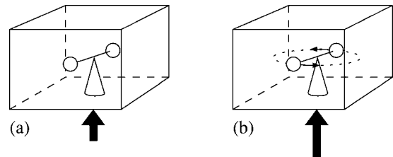
Fig. 13. A black box (transparent for clarity) containing a pair of balls that (a) are at rest and (b) are moving. The force needed to hold the box at a fixed height on Earth is greater when the balls are moving than when they are at rest. The force is proportional to the total relativistic energy of the box.
