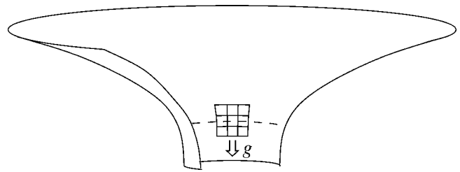
Fig. 4. A freely falling frame (the grid) accelerating relative to the spatial geometry of a black hole (Ref. 13). We consider circular motion along the dashed line. The bottom edge of the depicted surface corresponds to the horizon. At this edge the embedding approaches a cylinder and the circle at the horizon is thus straight in the sense that it does not curve relative to the surface.
