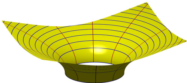
Fig. 19. A sketch of the apparent geometry of a symmetry plane through a black hole. The innermost circle is at the surface of the black hole.
