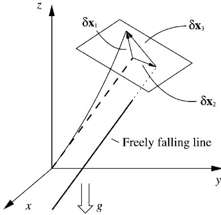
Fig. 14. Deviations from a straight line relative to the (properly) accelerated reference system. The z direction is chosen to be antiparallel to the local \mathbf{g} . The plane in which we study the deviations is perpendicular to the momentary direction of motion (the dashed line) and the three vectors lie in this plane. The solid curve is the particle trajectory as observed in the (properly) accelerated reference system. The thick line is a freely falling line that was aligned with the dashed line (and at rest relative to the reference frame) at the time when the particle was at the origin.
