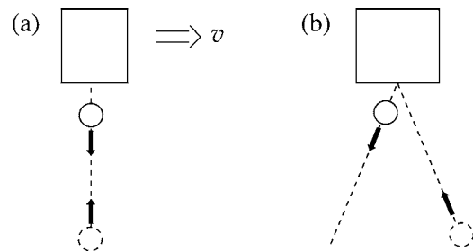
Fig. 8. A simple model where small particles bounce elastically on the object. (a) The scenario as observed from a system where the impulse giving particle has no horizontal velocity. (b) The corresponding scenario as observed from a system comoving with the object.
