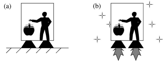
Fig. 20. (a) Dropping an apple inside an elevator on Earth gives the same motion relative to the elevator as (b) dropping it inside a (properly) accelerated elevator in outer space. In both cases we can introduce an inertial (fictitious) gravitational force—but there is (in either case) no real gravitational force (in Einstein's theory).
