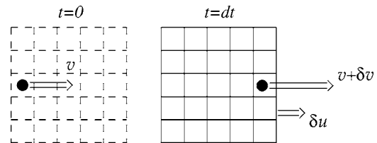
Fig. 15. An object moving relative to an accelerated reference frame. At t=0 the velocity of the particle is v . In a time \delta t the reference frame is accelerated to a velocity \delta u , and the velocity of the particle relative to the accelerated reference frame is v + \delta v .
