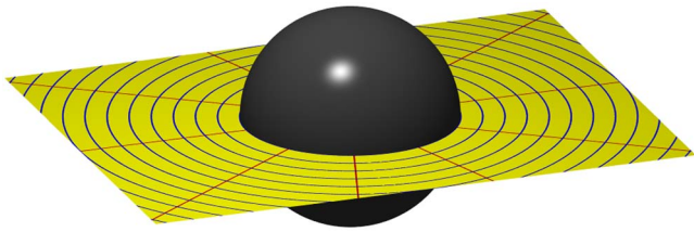
Fig. 18. A symmetry plane through a black hole.
