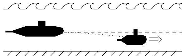
Fig. 10. A submarine submerged in a balanced state of rest in a flat ocean with proper upward acceleration will sink due to relativistic effects if it starts moving horizontally.
