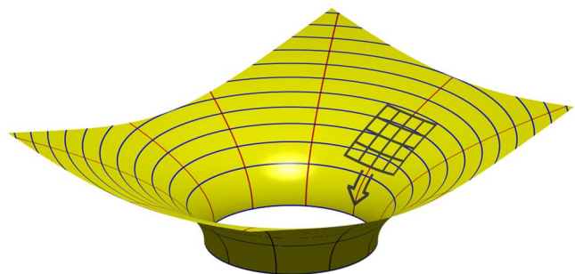
Fig. 21. A coordinate system accelerating (falling) relative to the curved spatial geometry of a black hole.
