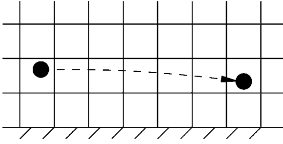
Fig. 5. A zoom-in on the circular motion observed from a static system (with proper upward acceleration). The trajectory curves slightly downward, which will decrease the upward acceleration of the object relative to a freely falling system. In the limit that the acceleration of the freely falling frames is infinite, we can disregard the small curvature.
