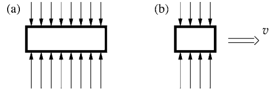
Fig. 9. (a) An idealized (rectangular) submarine submerged in water at rest relative to the water. (b) As the submarine moves, it will be length contracted and thus the given force from the water will decrease by a factor of \gamma .
