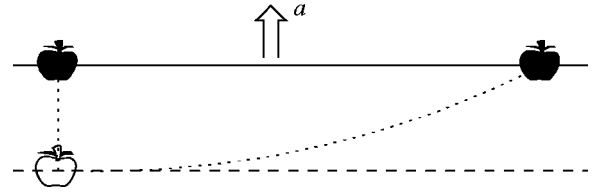
Fig. 3. Two apples on an upward accelerating line (the solid line). The apples were initially at the position of the unfilled apple, one at rest and the other moving horizontally to the right. Both apples have to move up the same amount for a given coordinate time. But the one that moves horizontally has less proper time to do it. It must therefore experience a greater acceleration.
