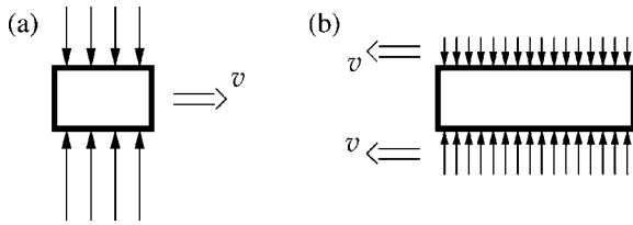
Fig. 11. (a) Observed from the water system the submarine is length contracted by a factor of \gamma . (b) Observed from the submarine the water columns are length contracted and thus denser by a factor of \gamma .
