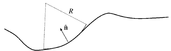
Fig. 17. A path on a plane always corresponds locally to a circle as far as direction and curvature are concerned.
