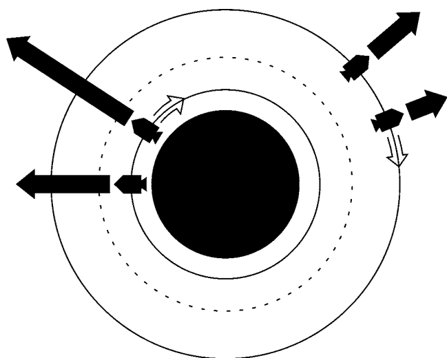
Fig. 1. Rockets orbiting a static black hole. The solid arrows correspond to the force (the rocket thrust) necessary to keep the rocket in circular orbit. Inside of the photon radius (the dashed circle), the required force increases as the orbital velocity increases.
